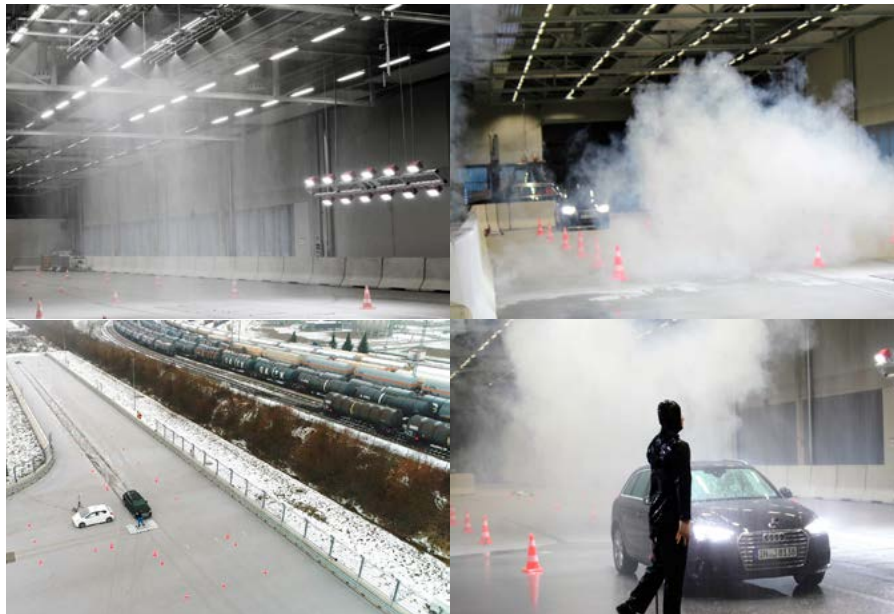
Outdoor and Indoor CARISSMA Test Facilities under weather conditions ( Rain and Fog Simulation Tests )
