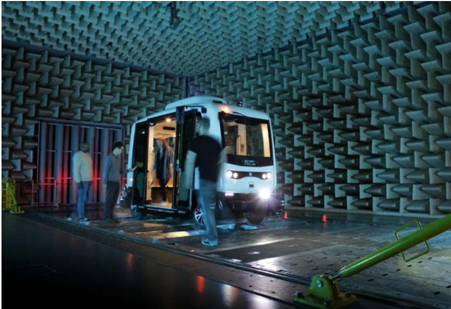
Autonomous shuttle in KIT's acoustic four-wheel roller dynamometer
